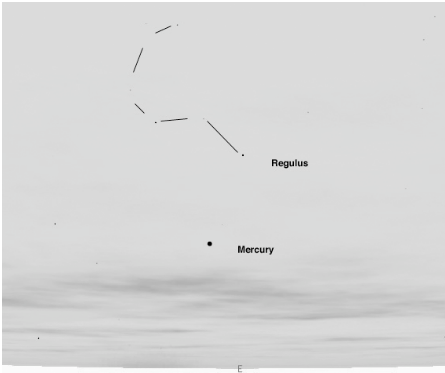
Mercury as seen in the east about 30 minutes before sunrise on September 19, 2010 from latitude 42°N.
